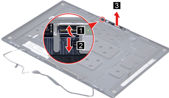
Figure 39. Remove the camera board
