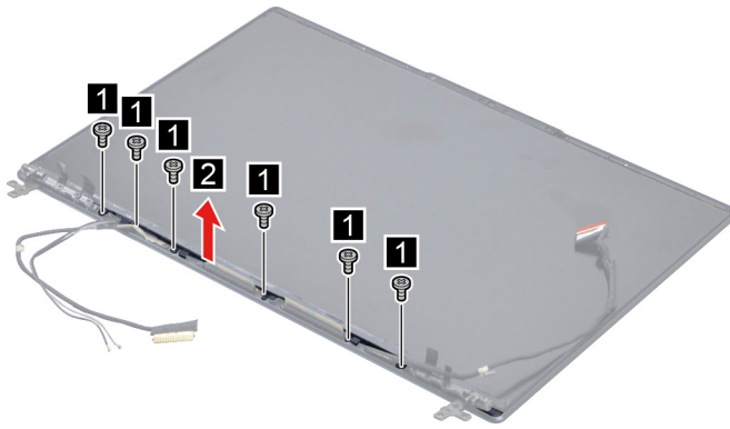
Figure 45. Remove the strip cover
