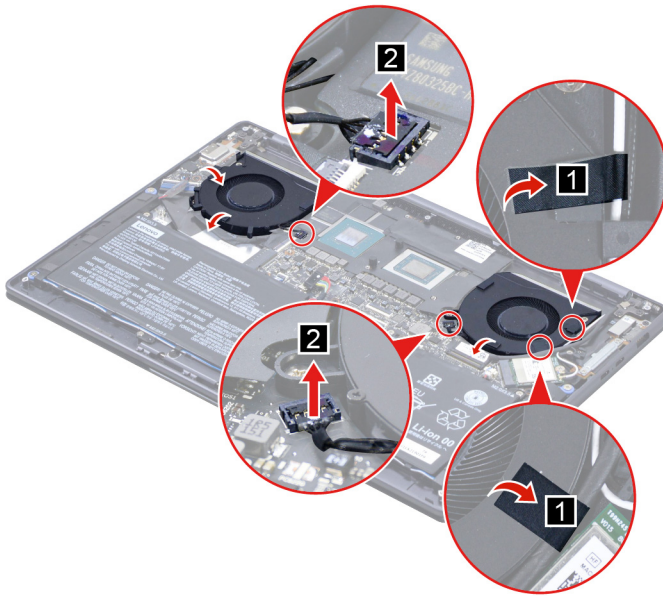
Figure 18. Disconnect the fan cables from the system board
