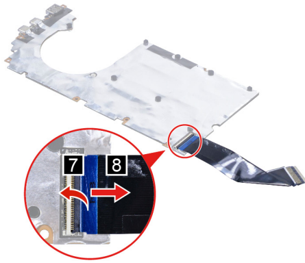
Figure 28. Remove the I/O board cable
