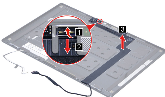
Figure 40. Remove the camera cable
