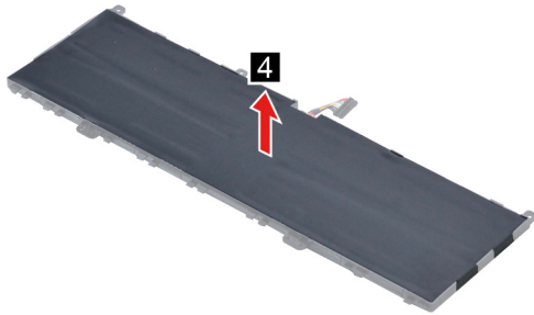
Figure 7. Remove the battery pack mylar
