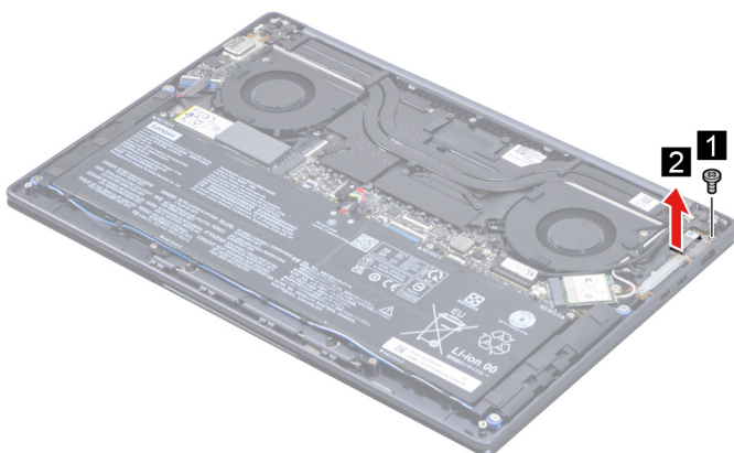
Figure 15. Remove the system-USB board shielding
