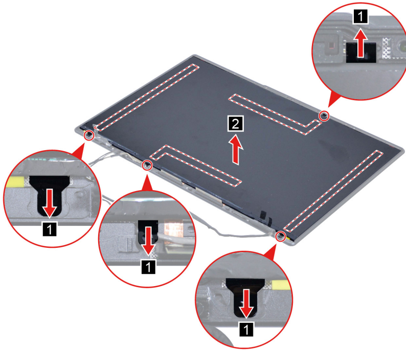
Figure 46. Remove the LCD panel
