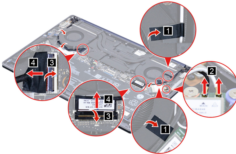
Figure 29. Disconnect cables
