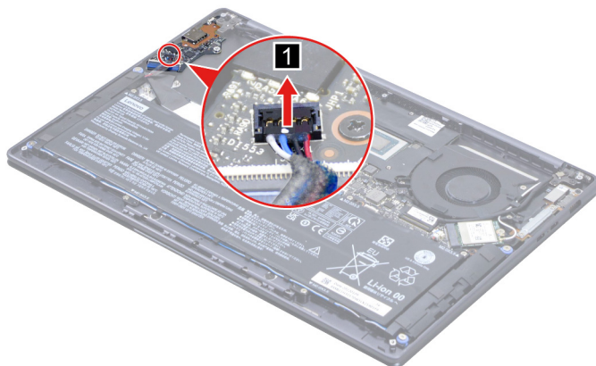
Figure 24. Disconnect the speaker cable from the I/O board
