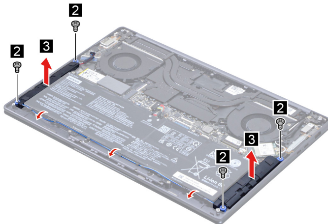
Figure 21. Remove the speakers
