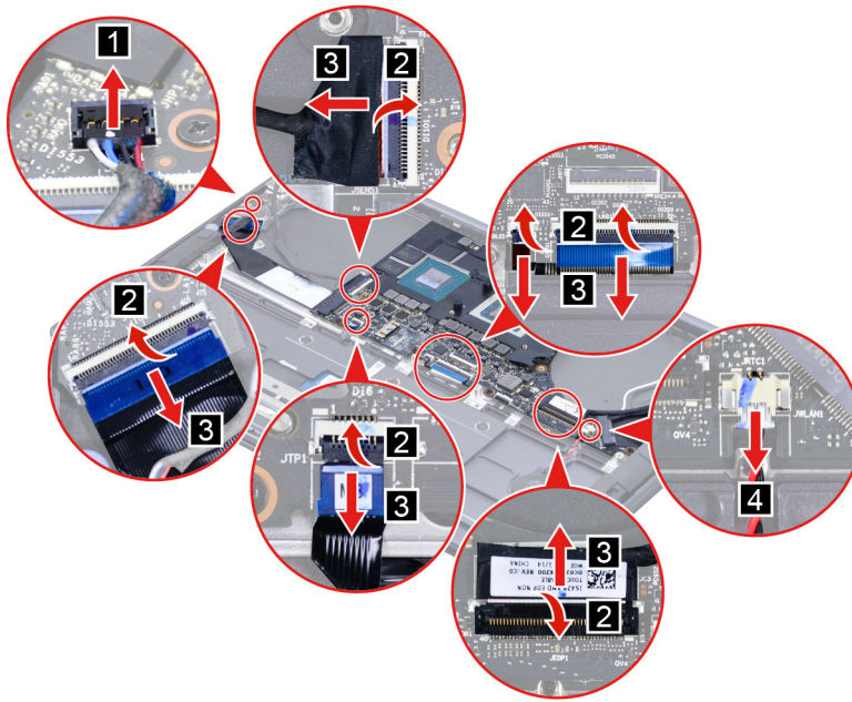
Figure 26. Disconnect cables connected to the system board
