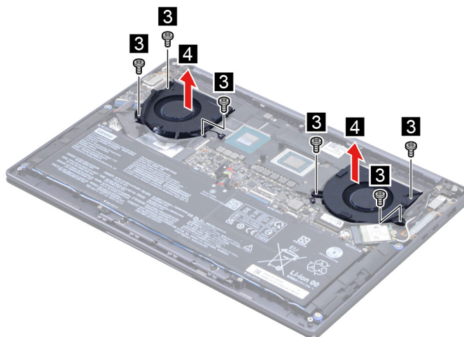
Figure 19. Remove the fans
