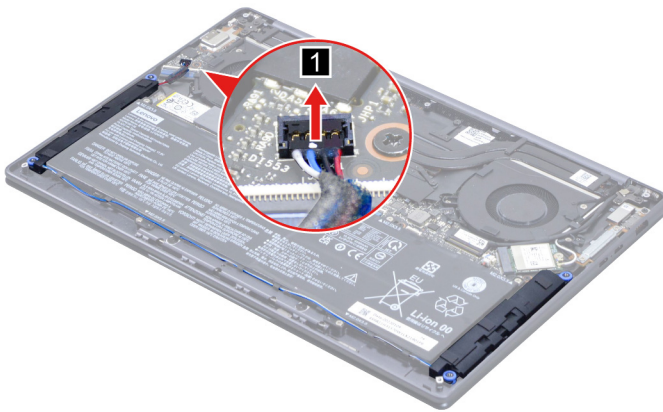
Figure 20. Disconnect the speaker cable from the system board
