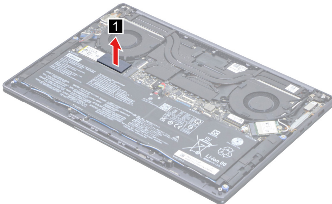
Figure 8. Remove the SSD thermalpad
