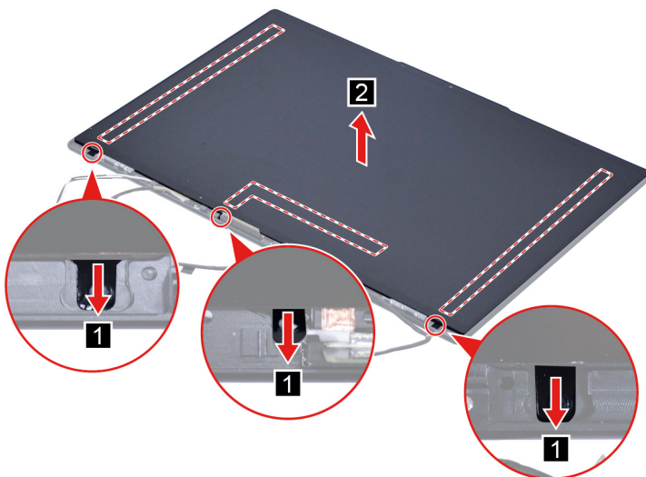
Figure 35. Remove the LCD panel
