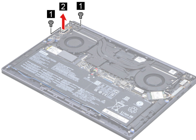
Figure 14. Remove the I/O board shielding
