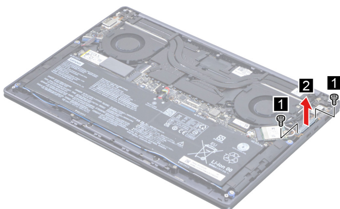
Figure 16. Remove the Type-C bracket
