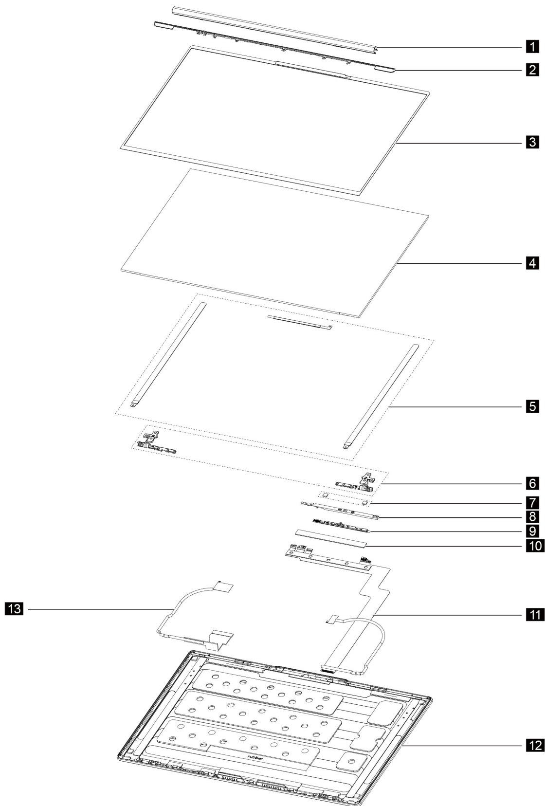
Figure 3. LCD module (mylar) — exploded view
