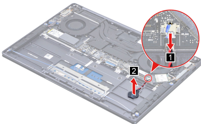
Figure 23. Remove the CMOS battery
