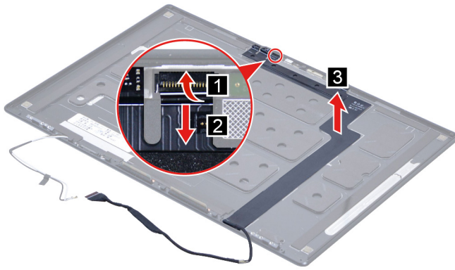
Figure 50. Remove the camera cable
