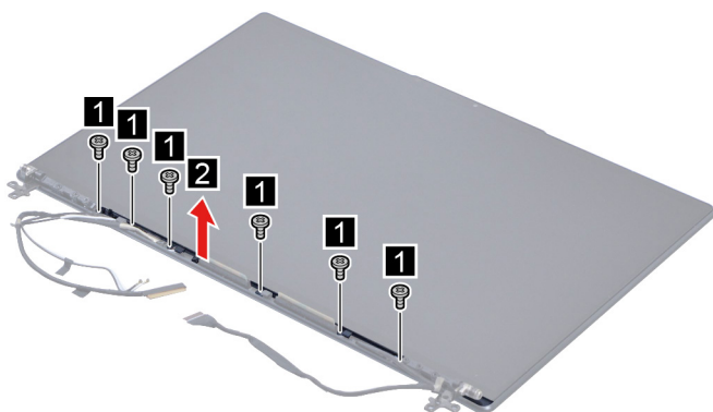
Figure 34. Remove the strip cover
