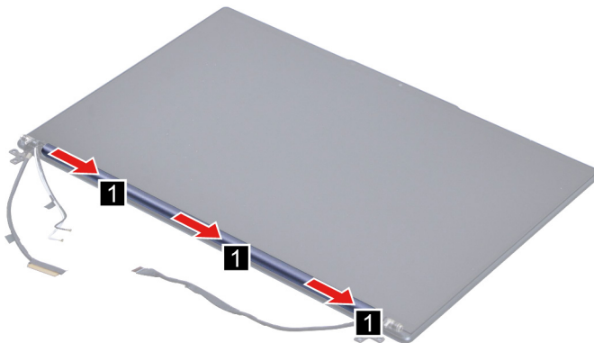
Figure 31. Remove the hinge cover
