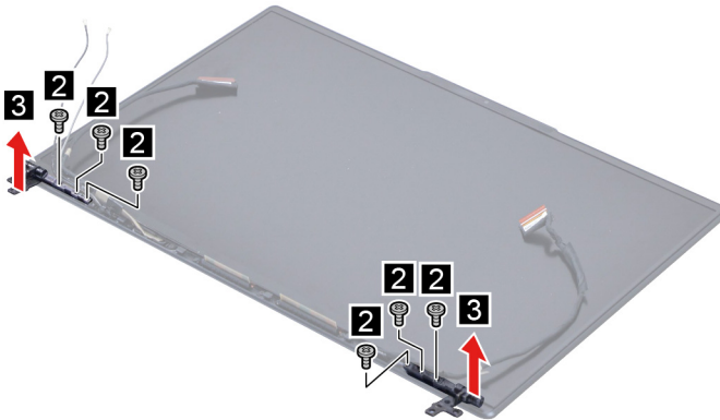
Figure 44. Remove eight screws and then remove the hinges
