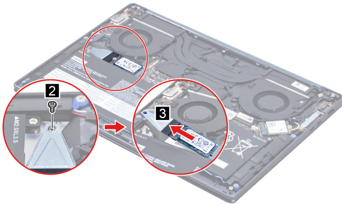
Figure 11. Remove the SSD
