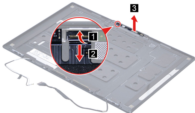
Figure 49. Remove the camera board
