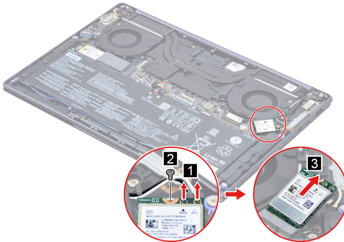
Figure 13. Remove the Wi-Fi card
