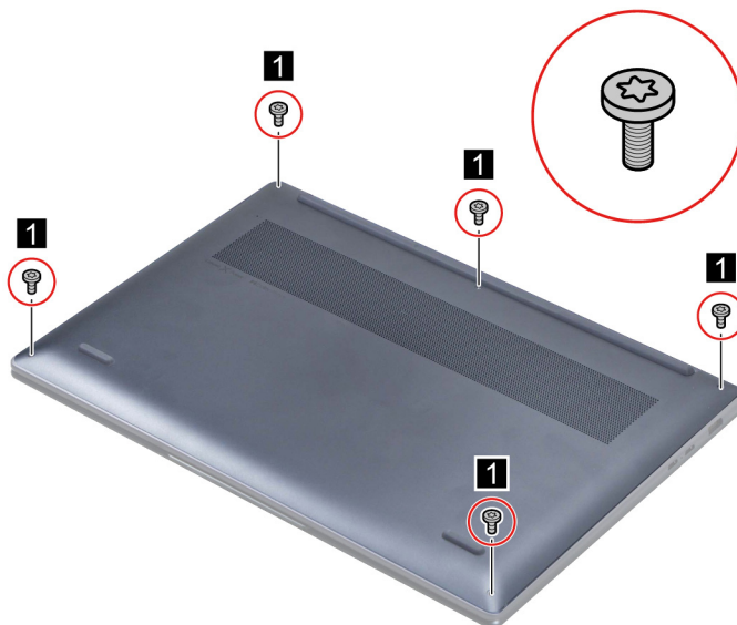
Figure 4. Remove five screws
