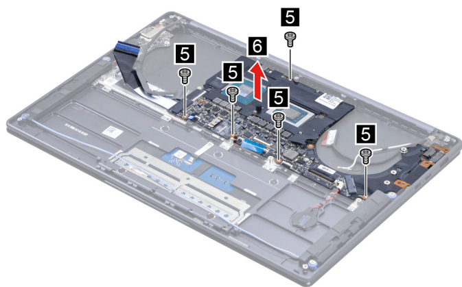
Figure 27. Remove the system board with the I/O board cable
