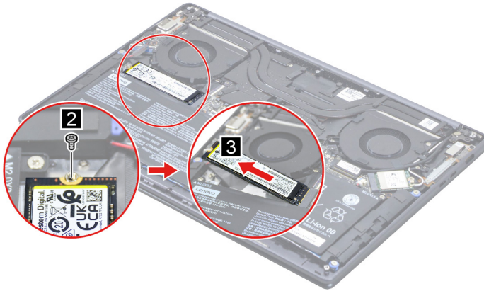
Figure 9. Remove the SSD
