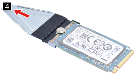
Figure 12. Remove the SSD bracket
