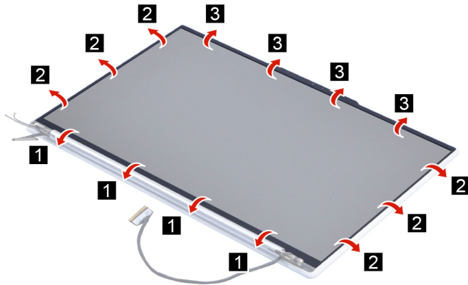
Figure 26. Remove the LCD bezel
