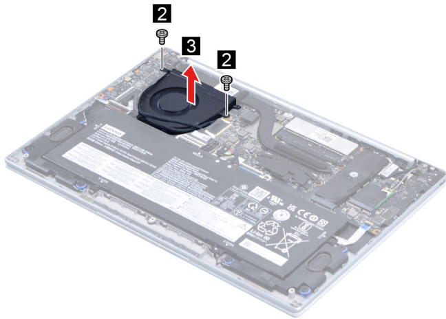
Figure 11. Remove two screws then remove the fan.
