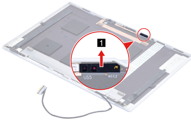
Figure 34. Remove the ToF rubber
