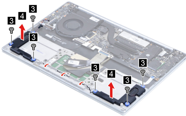
Figure 19. Remove the six screws then remove the speakers.
