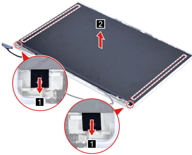
Figure 30. Remove LCD panel
