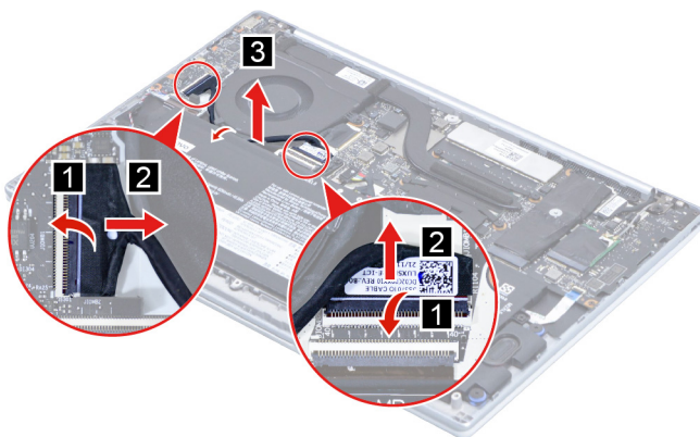
Figure 16. Remove I/O board cable
