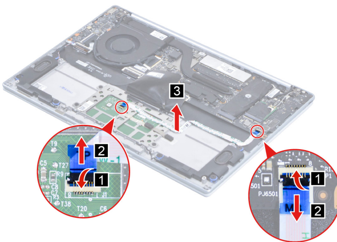
Figure 20. Remove the touchpad board cable
