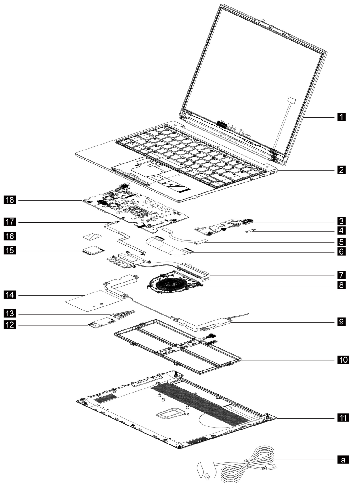
Figure 1. Lenovo Slim 7 Carbon 13IAP7 exploded view
