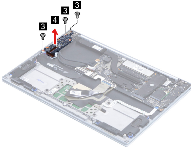
Figure 15. Remove three screws then remove the I/O board
