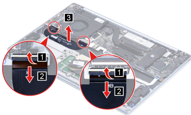
Figure 17. Remove I/O board FPC
