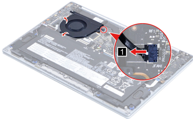
Figure 10. Disconnect the fan cable from the system board
