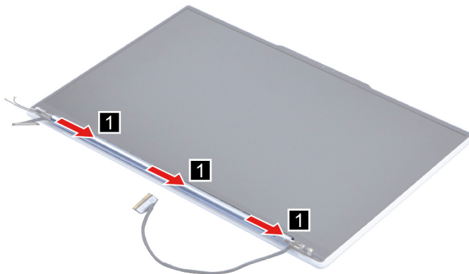
Figure 25. Remove the hinge cover
