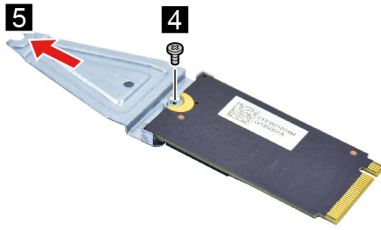
Figure 8. Remove one screw then remove the SSD bracket
