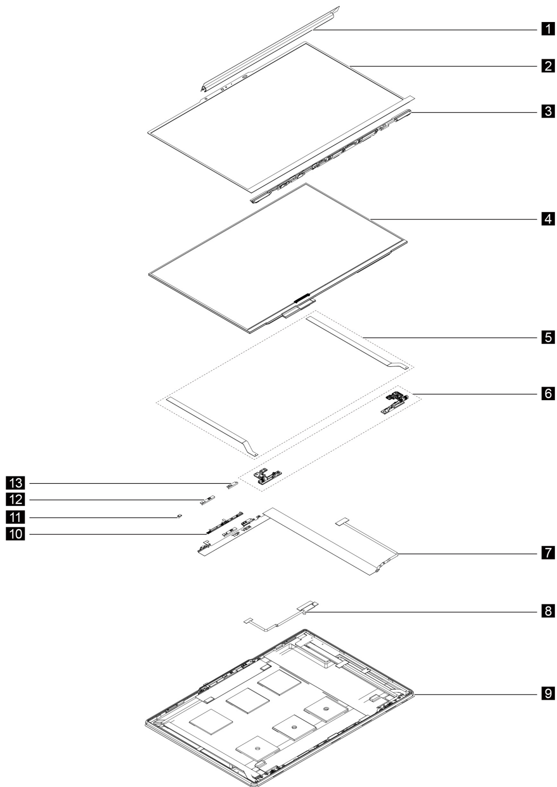
Figure 2. Lenovo Slim 7 Carbon 13IAP7 LCD module — exploded view
