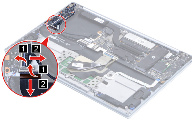
Figure 14. Disconnect cables connected to the I/O board
