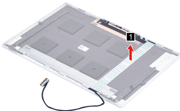
Figure 35. Remove two screws and then remove the camera bracket
