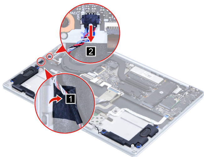
Figure 18. Disconnect the speaker cable connector from the I/O board
