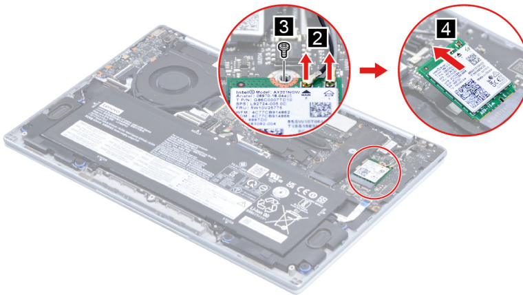
Figure 12. Remove the Wi-Fi card
