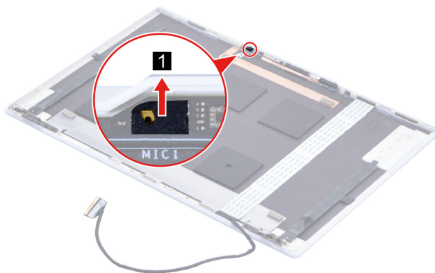
Figure 32. Remove the microphone rubber
