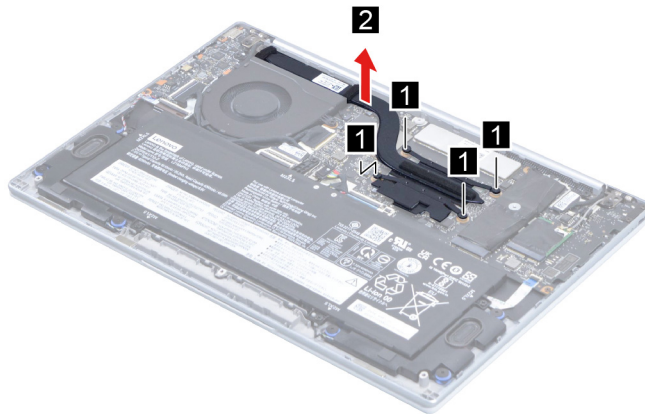
Figure 9. Remove the heat sink
