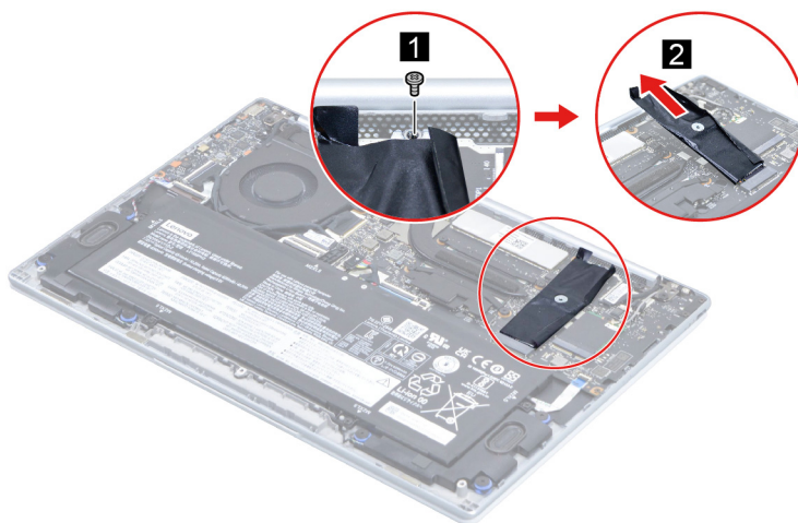
Figure 6. Remove the SSD with SSD bracket
