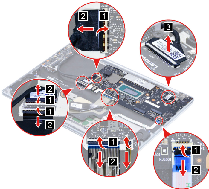
Figure 21. Disconnect cables connected to the system board
