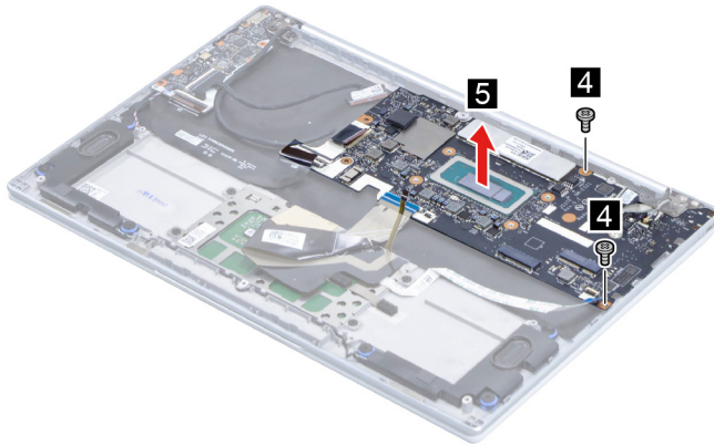
Figure 22. Remove two screws and then remove the system board
