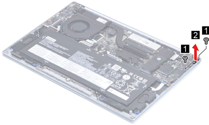
Figure 13. Remove the two screws then remove the Type-C bracket
