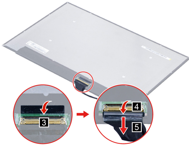
Figure 31. Detach the EDP cable
