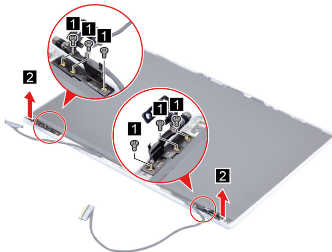
Figure 29. Remove six screws then remove the hinges
