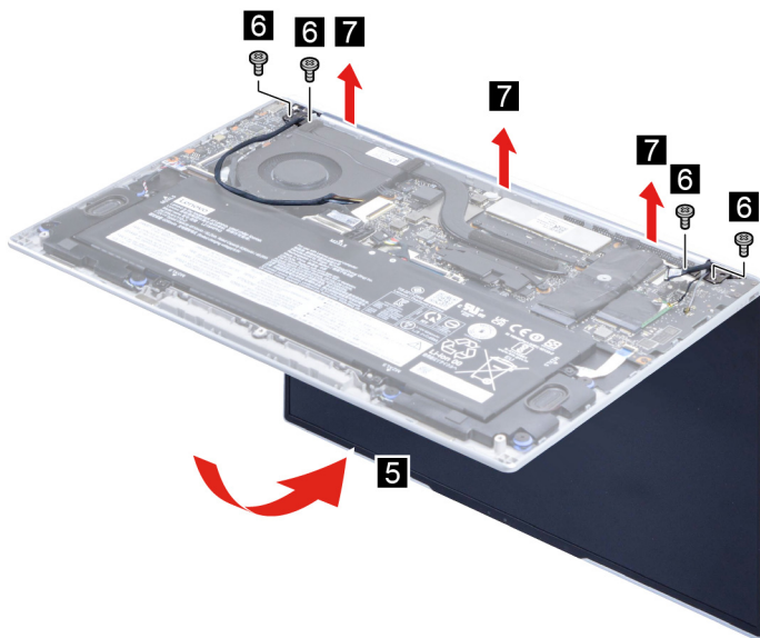
Figure 24. Remove the LCD module
