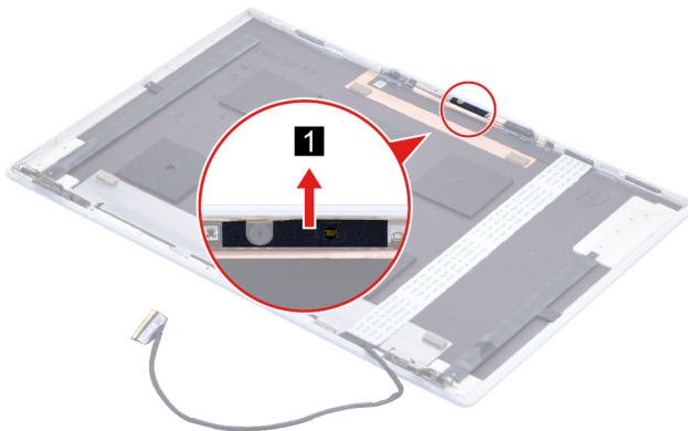
Figure 33. Remove the camera rubber
