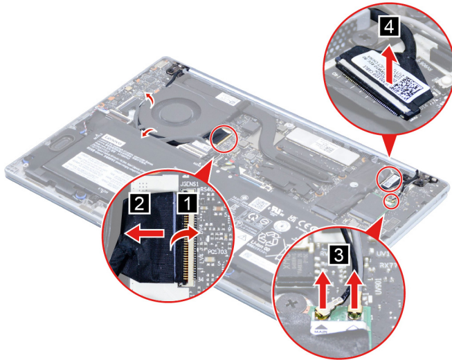
Figure 23. Disconnect the camera board cable, EDP cable and antenna cable
