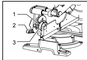
1. Pointer 2. Lever 3. Bevel scale plate
