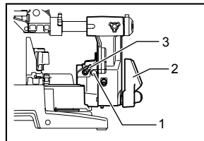
1. 0° Angle adjusting bolt 2. Lever 3. Latch lever
