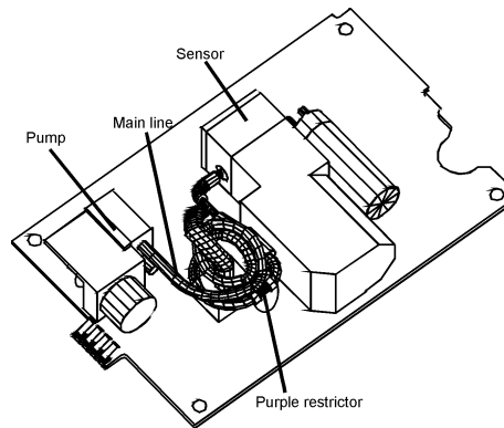
Figure 7-8: Main line
