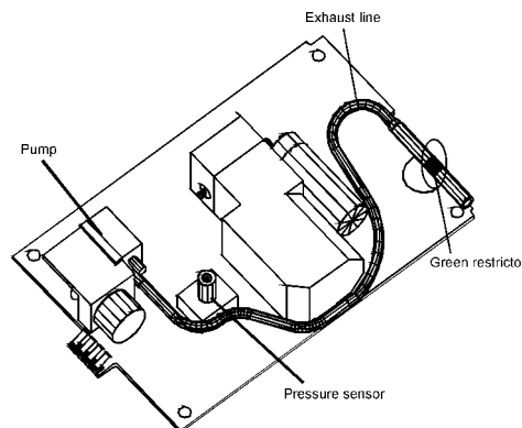
Figure 7-9: Exhaust line
